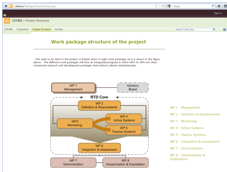
Figure 4: Project Structure
